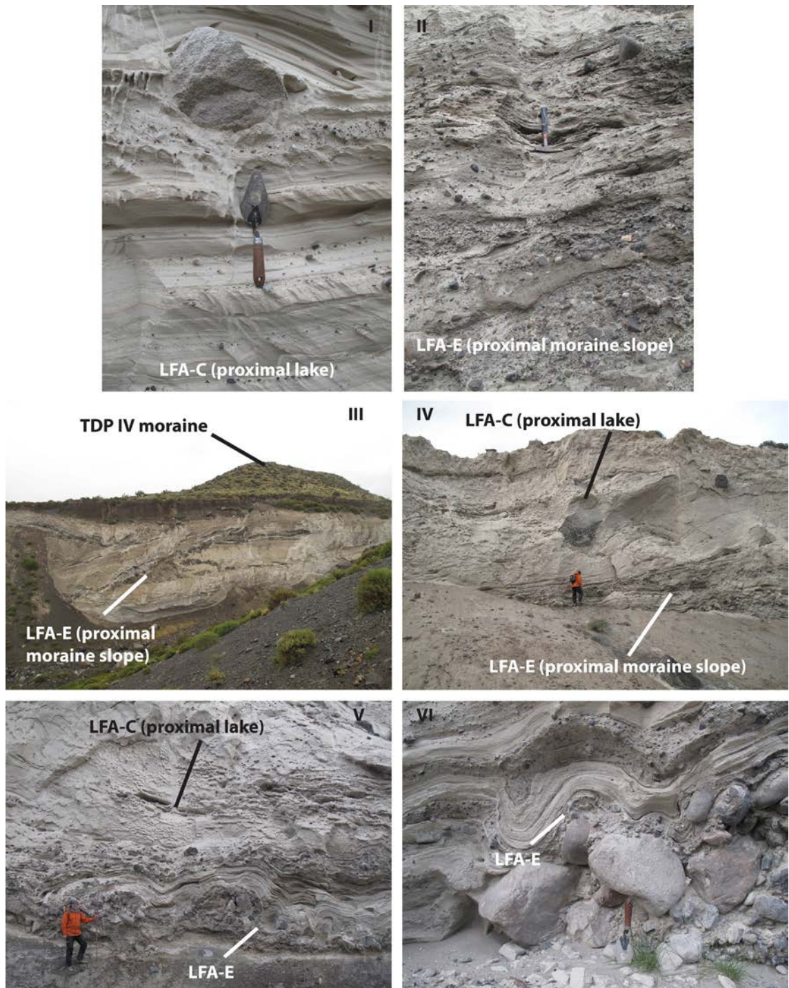
FIG. 4. Sediment facies associations (LFA) in El Canal stratigraphic section. I. composite sediment of LFA-C, including interlayered ice rafted debris (IRD), traction gravels and draped silt; II. Deformed proximal subaqueous outwash and mass flow deposits of LFA-E; III. Stratigraphic section vi with the TDP IV moraine ridge at the surface of the site (section is about 7 m high); IV. Glaciolacustrine sediments, including IRD (note big dropstone at the center of the photograph), overlying diamictons of LFA-E, west of stratigraphic section vi; V-VI. folded gravel beds of LFA-E, west of stratigraphic section vi (spatula is about 30 cm).
