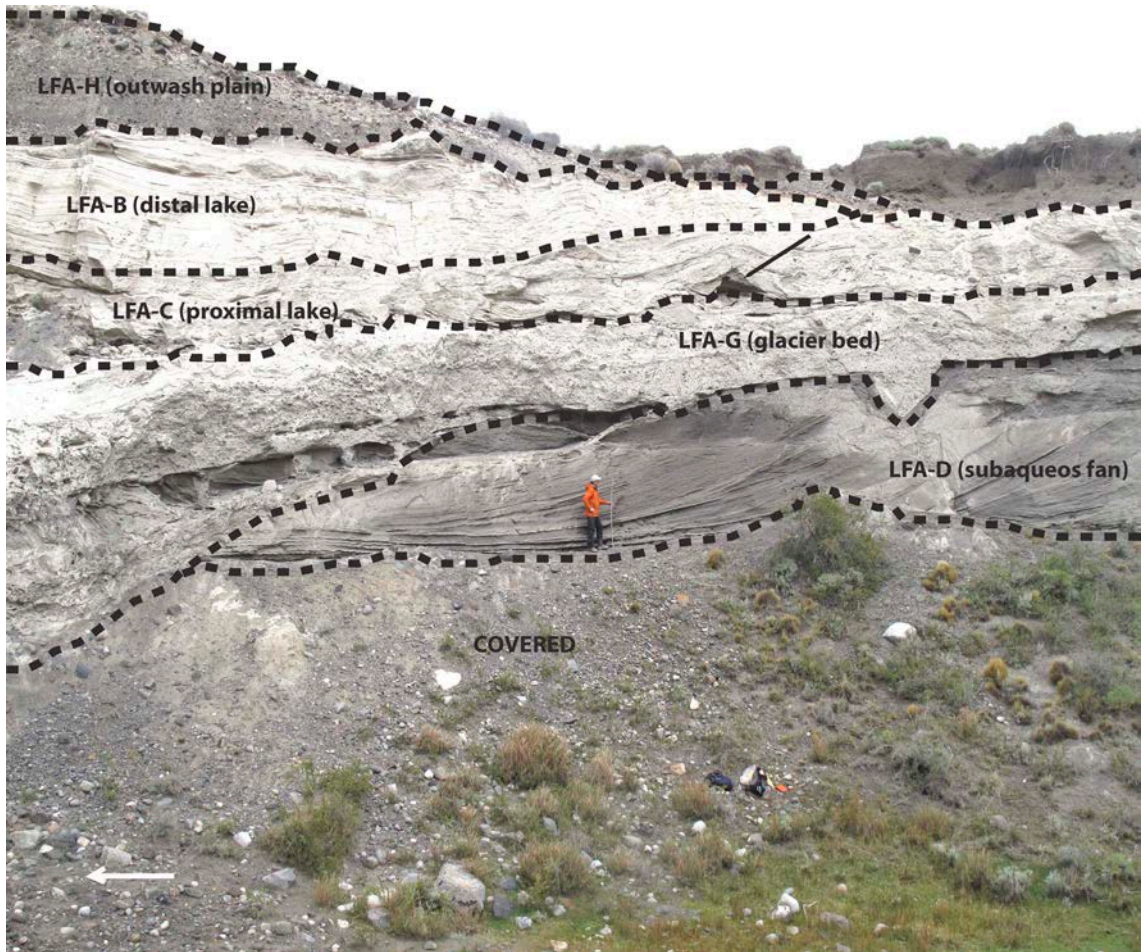
FIG. 8. Stratigraphic section iv. Black arrow points to iceberg dump deposits within lithofacies association C. View is to the south. White arrow indicates ice flow direction.
